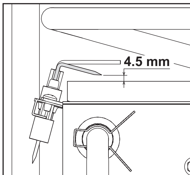
fig. 16 - Electrode position
